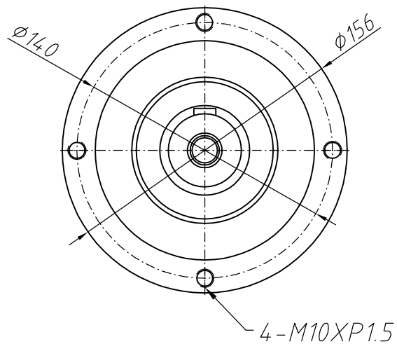
Output shaft
