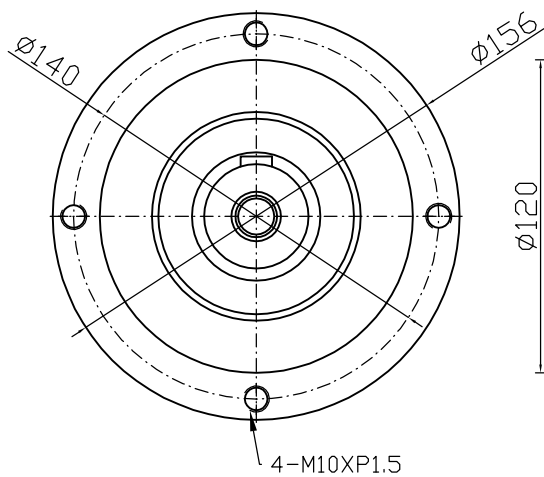
Output shaft
