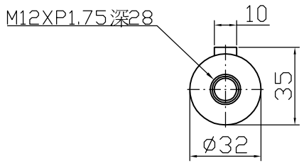
Output shaft
