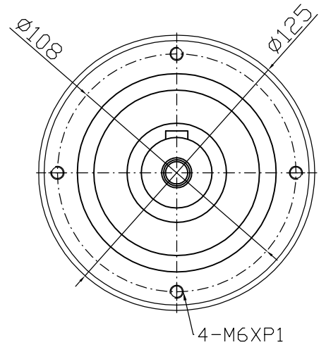
Output shaft
