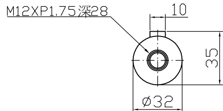
Output shaft
