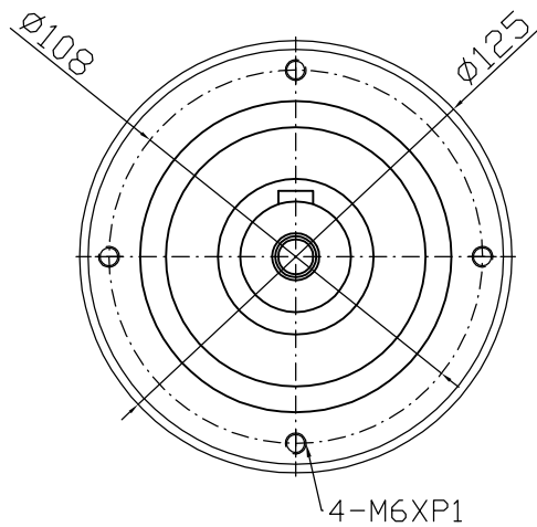
Output shaft
