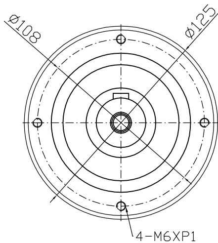
Output shaft
