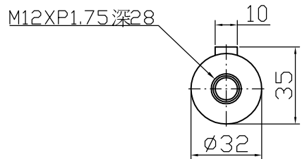
Output shaft
