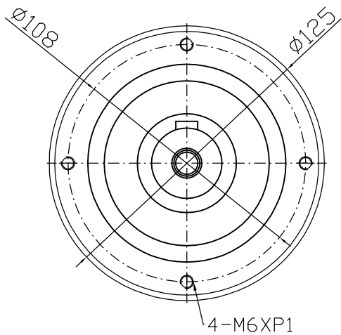
Output shaft
