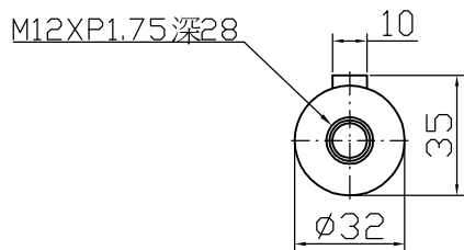
Output shaft
