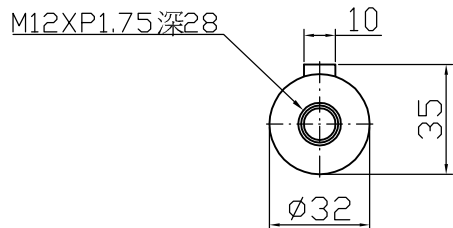
Output shaft
