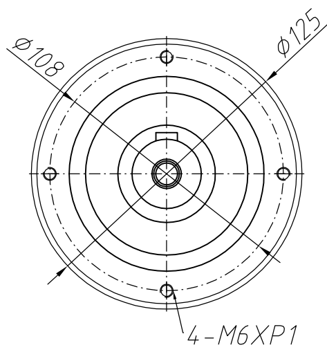
Output shaft
