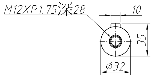
Output shaft
