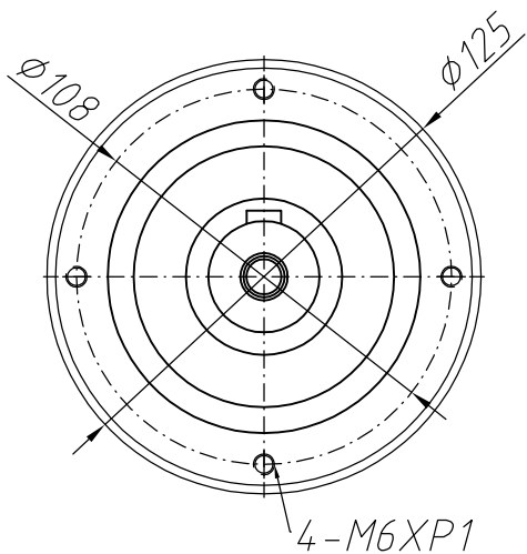
Output shaft
