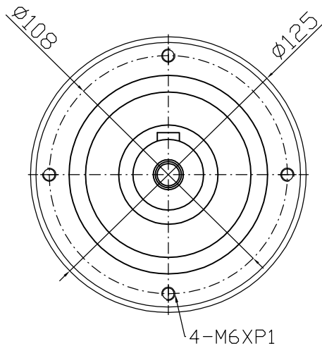
Output shaft
