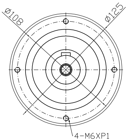
Output shaft
