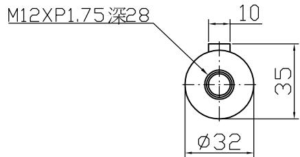
Output shaft
