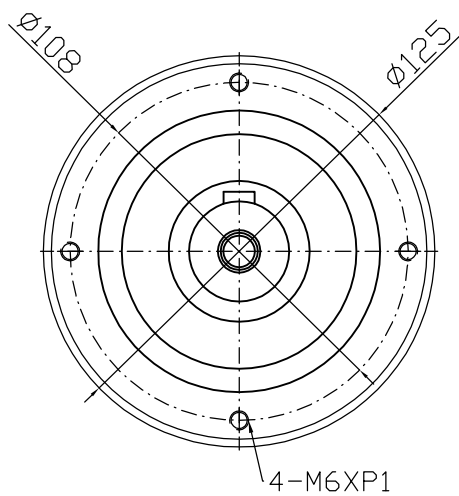
Output shaft
