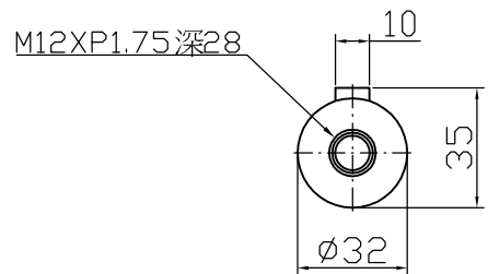
Output shaft
