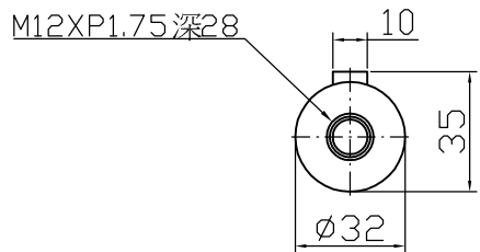
Output shaft
