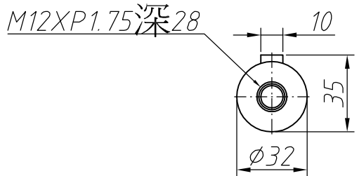
Output shaft
