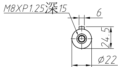
Output shaft
