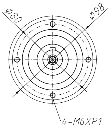
Output shaft
