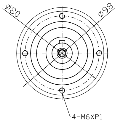
Output shaft
