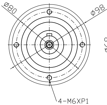
Output shaft
