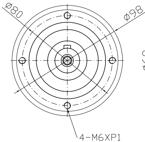
Output shaft
