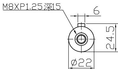
Output shaft
