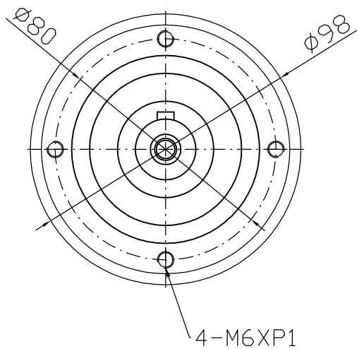
Output shaft
