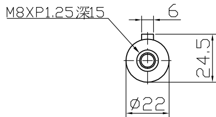
Output shaft
