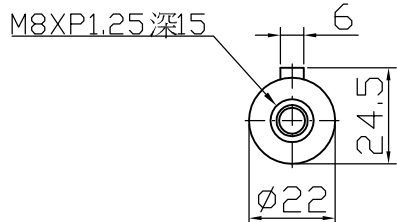
Output shaft
