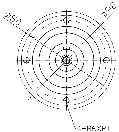
Output shaft
