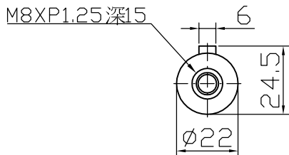
Output shaft
