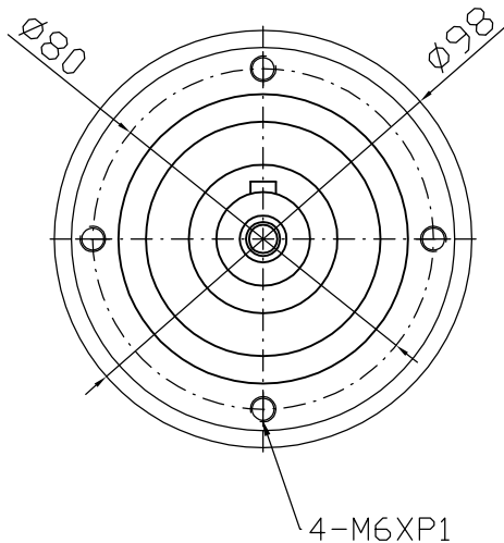
Output shaft
