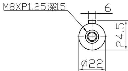
Output shaft
