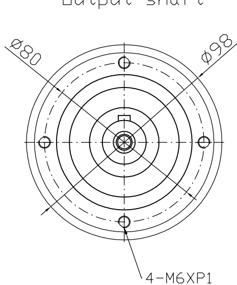
Output shaft
