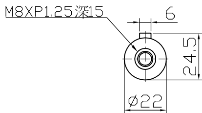
Output shaft
