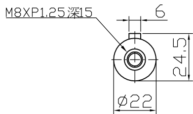
Output shaft
