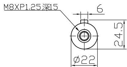
Output shaft
