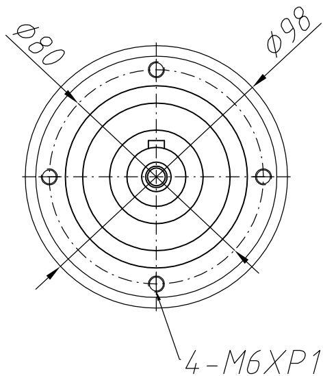
Output shaft
