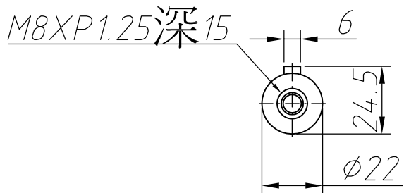
Output shaft
