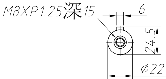
Output shaft
