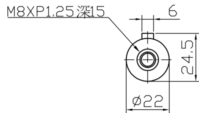
Output shaft
