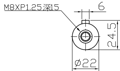
Output shaft
