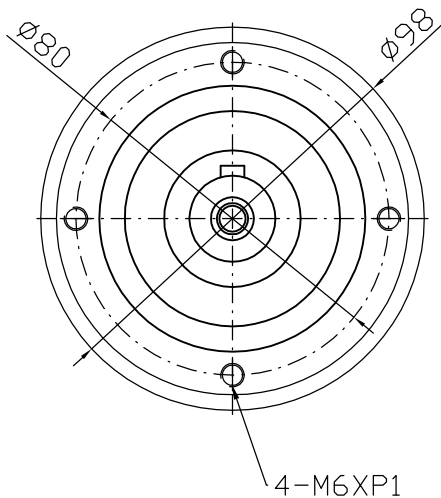
Output shaft
