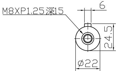
Output shaft
