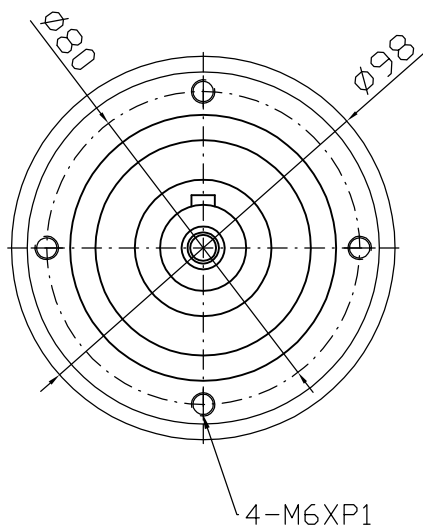
Output shaft
