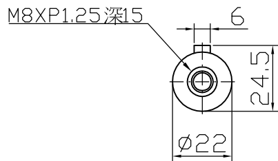
Output shaft
