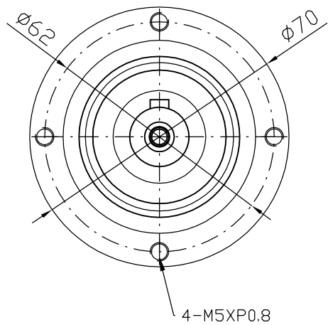
Output shaft
