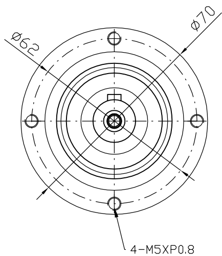
Output shaft
