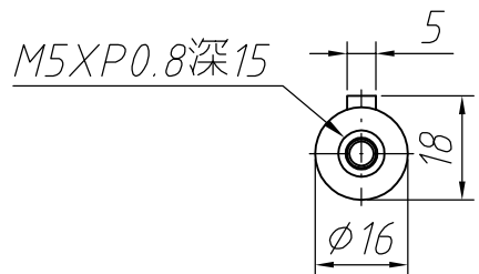
Output shaft
