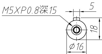
Output shaft
