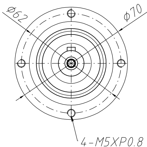
Output shaft
