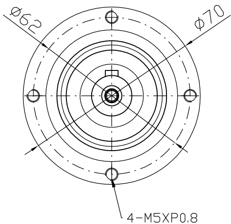
Output shaft
