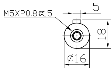
Output shaft
