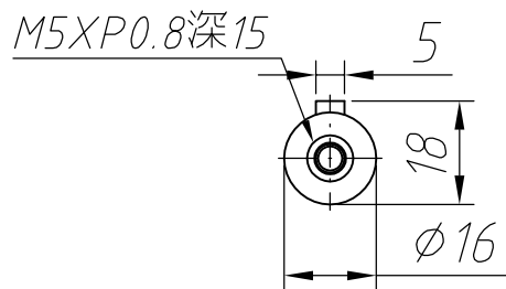
Output shaft
