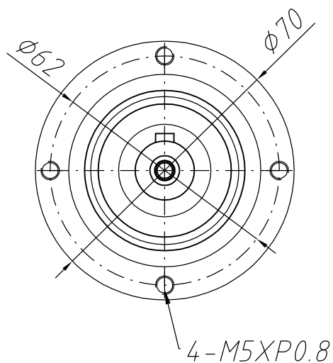
Output shaft
