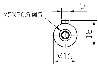
Output shaft
