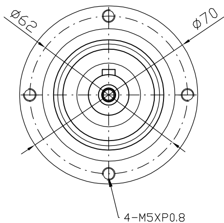
Output shaft
