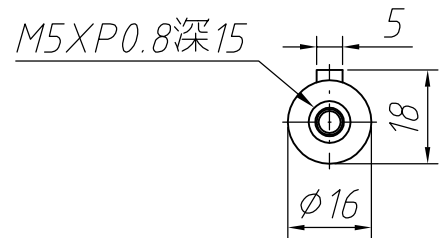
Output shaft
